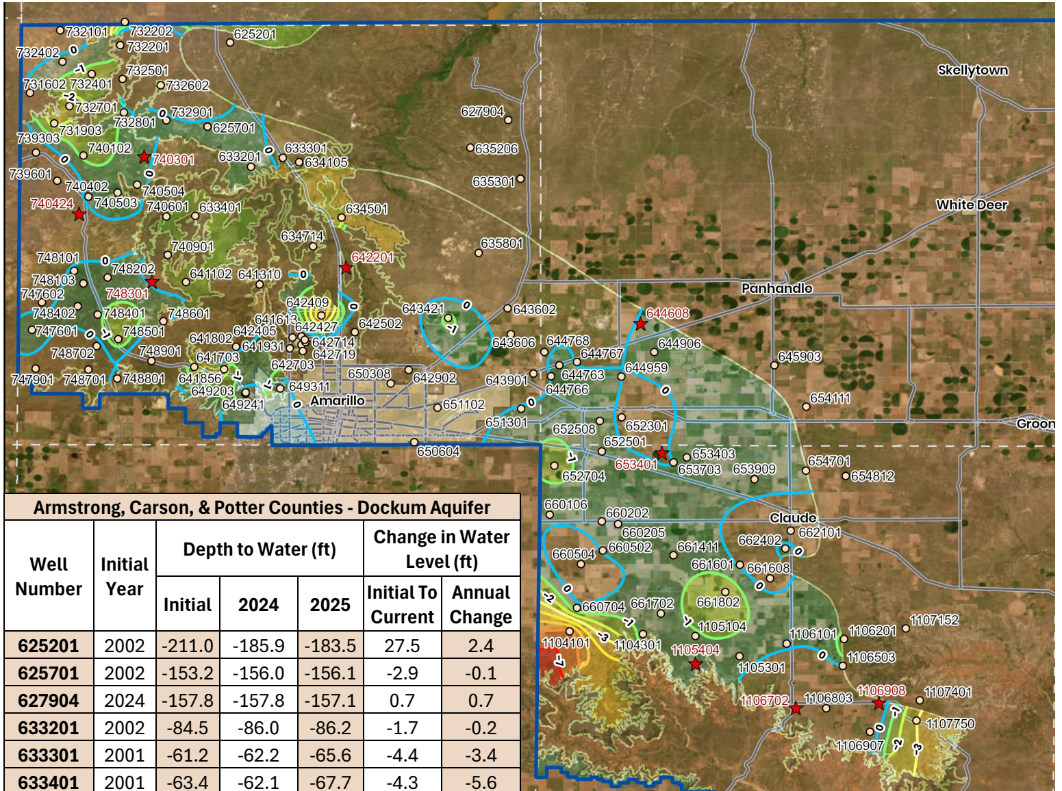
Armstrong, Carson, & Potter Counties - Dockum Aquifer
