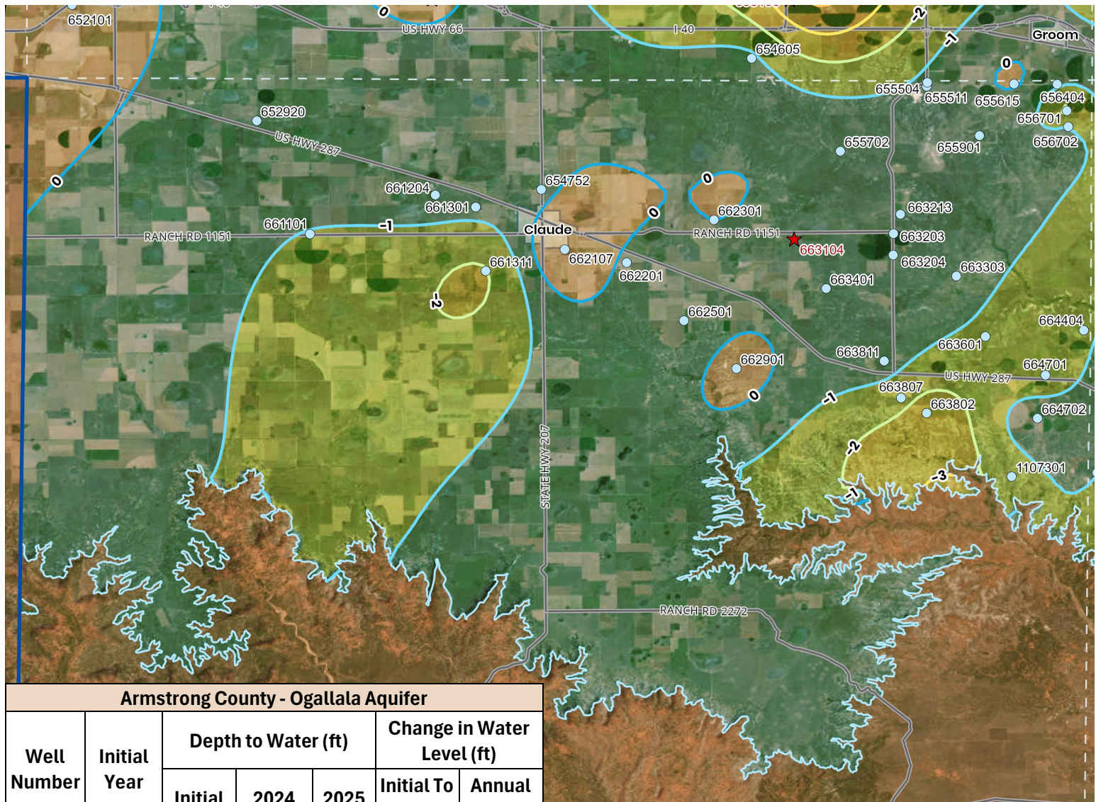
Armstrong County - Ogallala Aquifer
