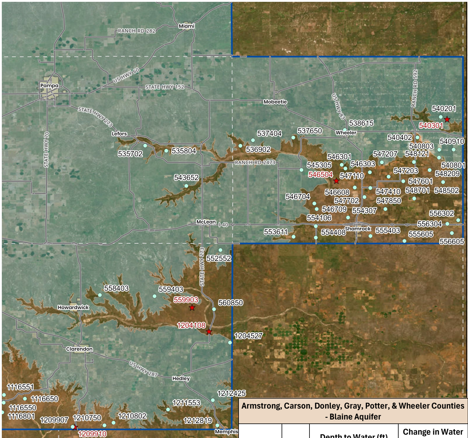
Armstrong, Carson, Donley, Gray, Potter, & Wheeler Counties - Blaine Aquifer
