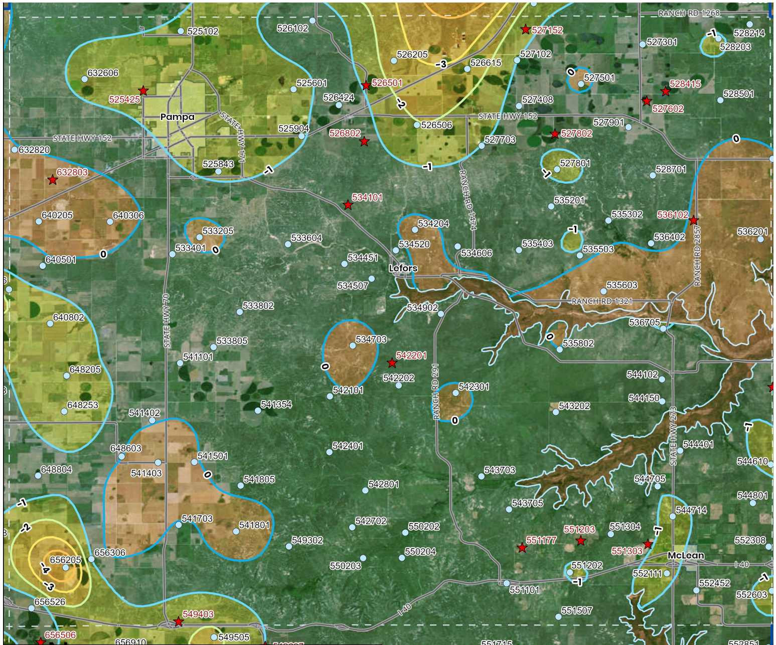
Gray County - Ogallala Aquifer
