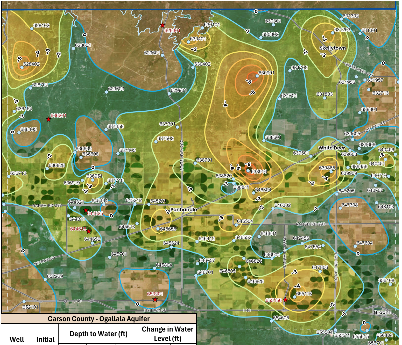
Carson County - Ogallala Aquifer
