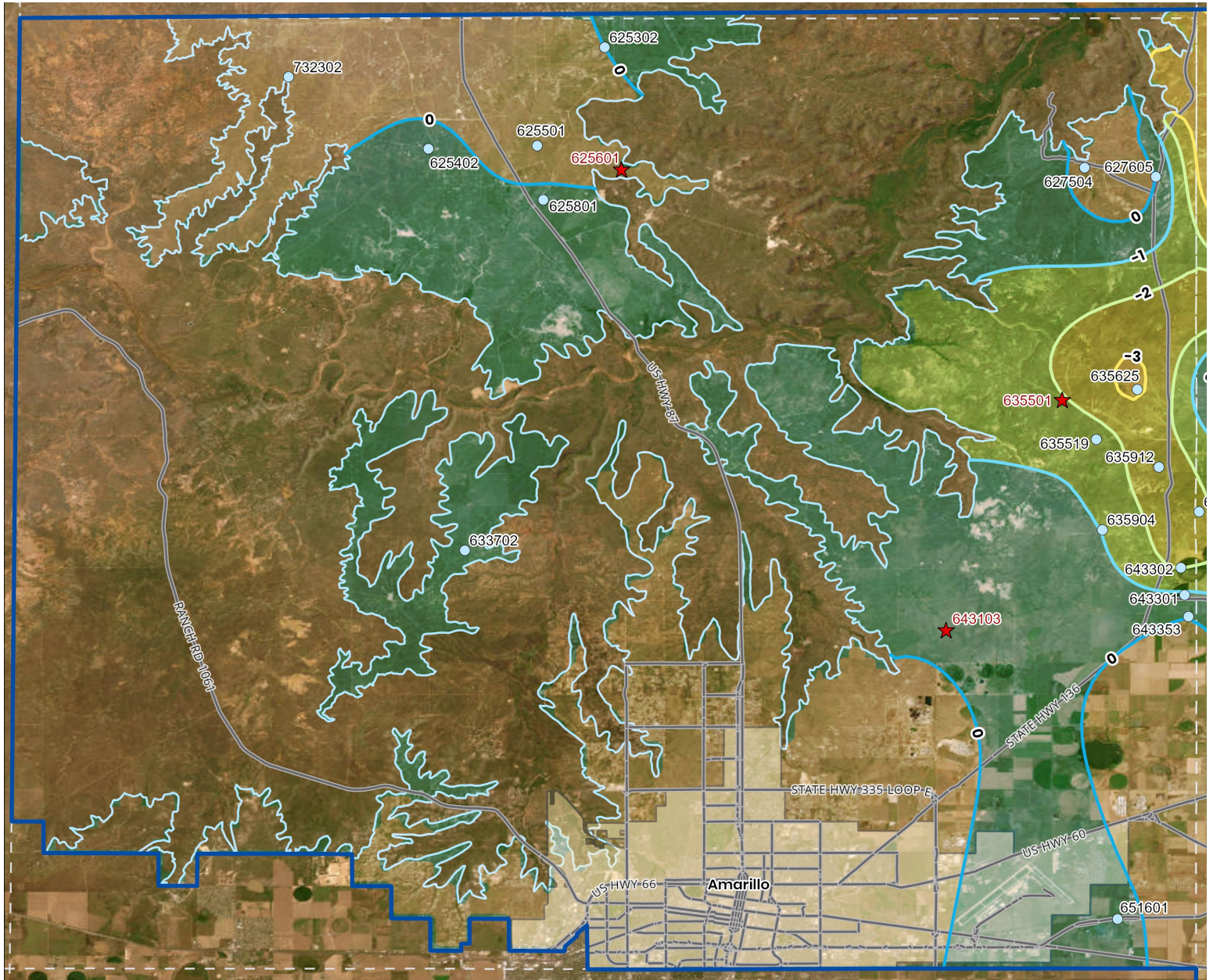
Potter County - Ogallala Aquifer
