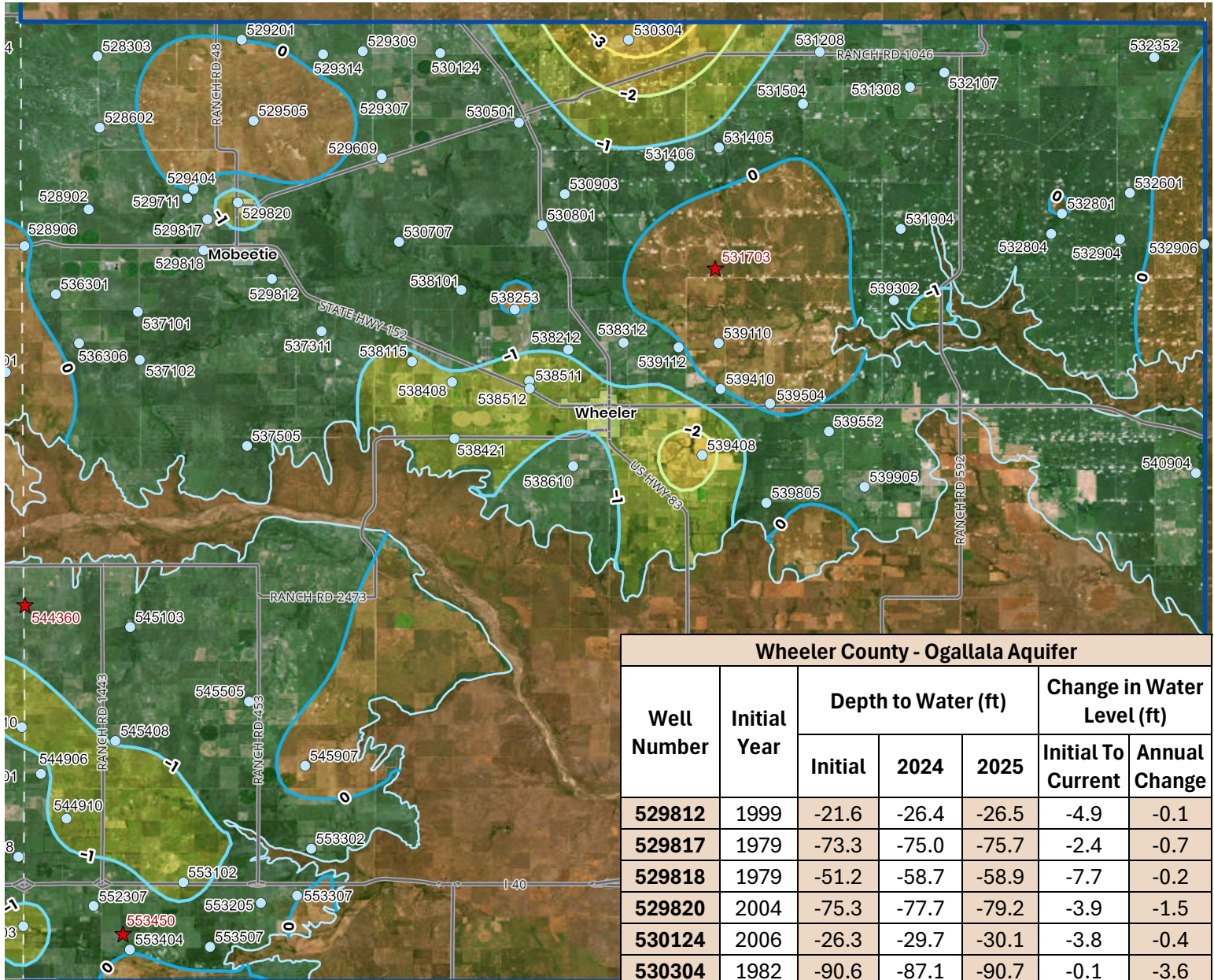
Wheeler County - Ogallala Aquifer
