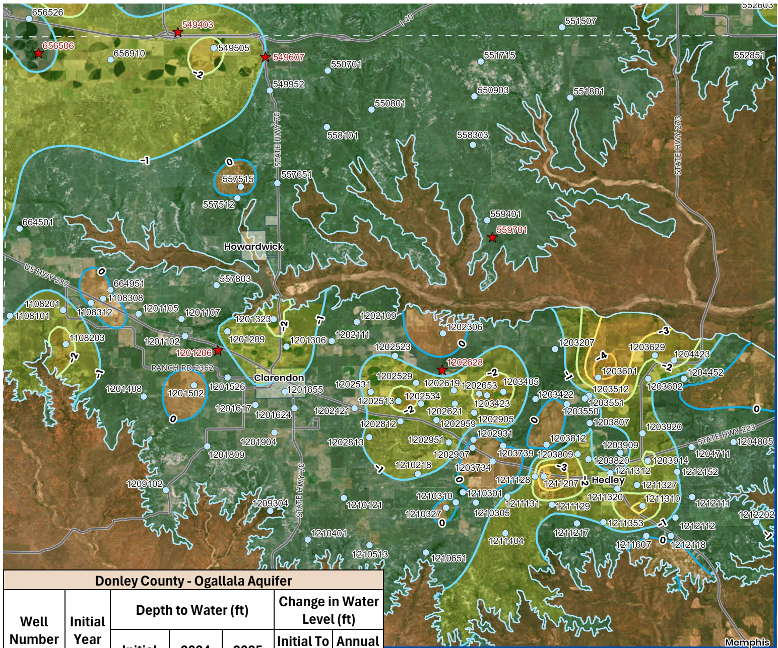
Donley County - Ogallala Aquifer
